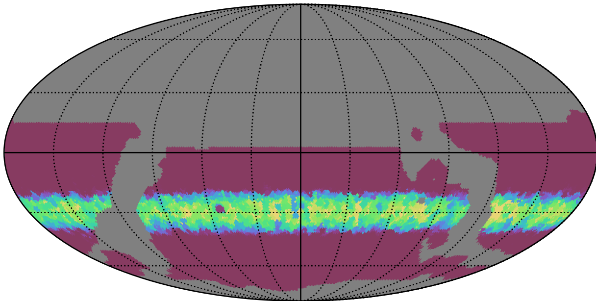
weather_cloudso8v3.4_10yrs WFD r band: Min normairmass
