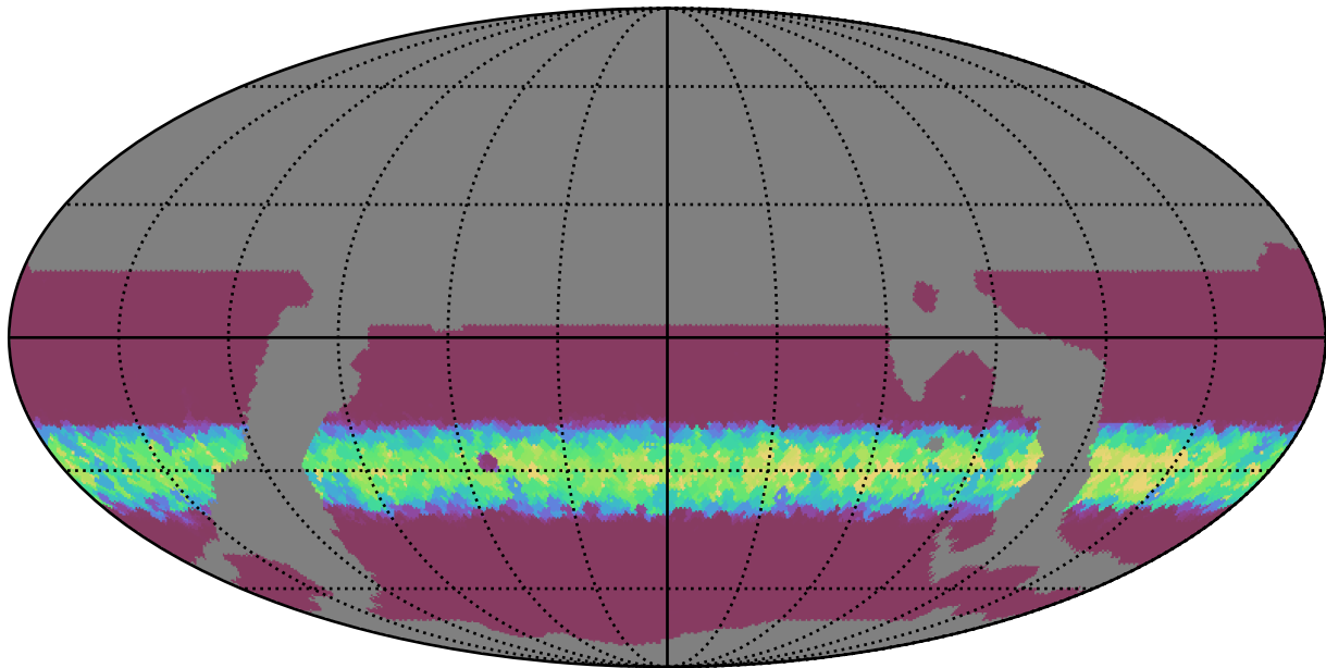
weather_cloudso8v3.4_10yrs WFD i band: Min normairmass
