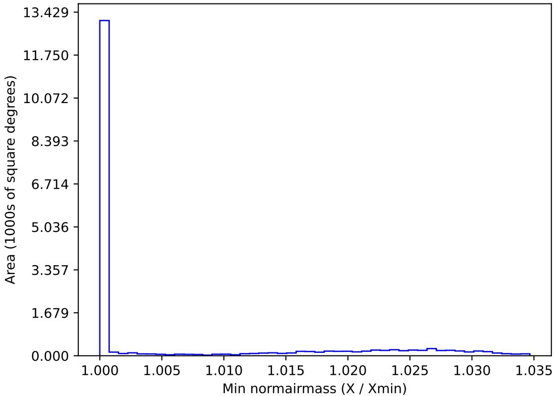
weather_cloudso8v3.4_10yrs WFD i band: Min normairmass
