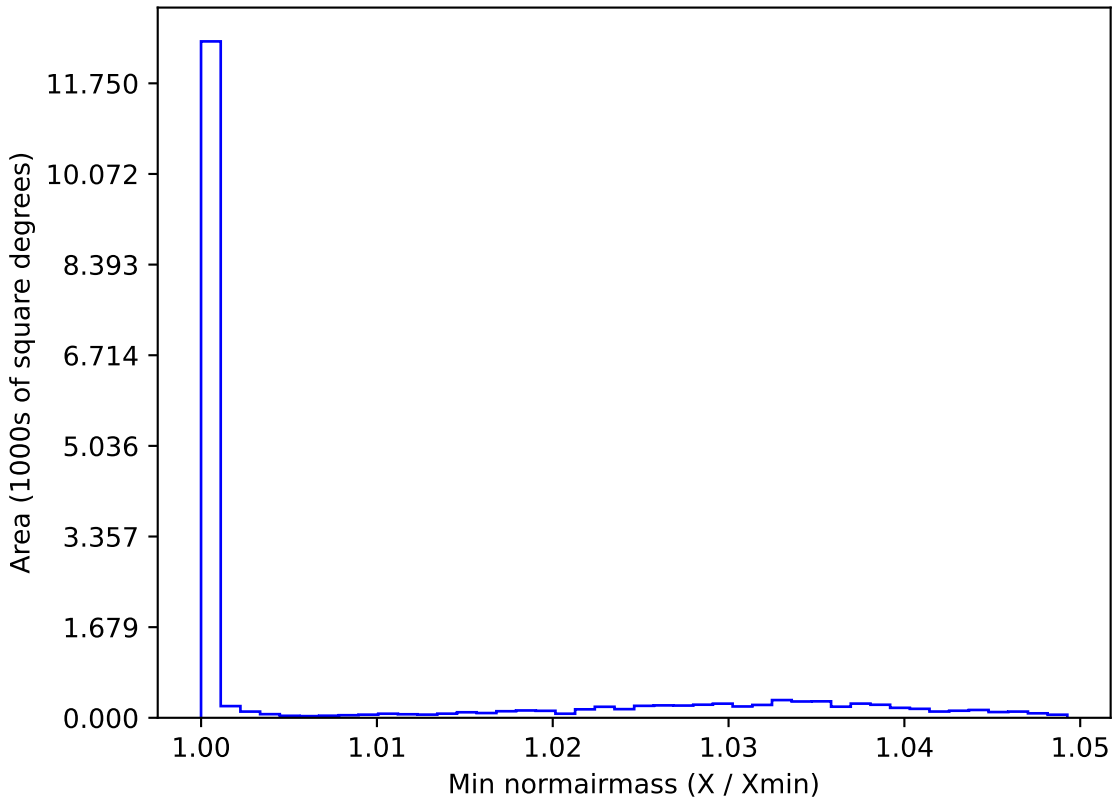
weather_cloudso8v3.4_10yrs WFD g band: Min normairmass
