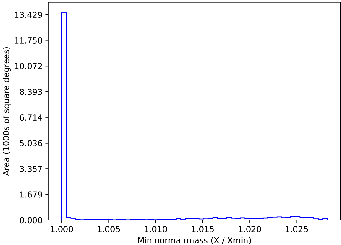
weather_cloudso8v3.4_10yrs WFD all bands: Min normairmass
