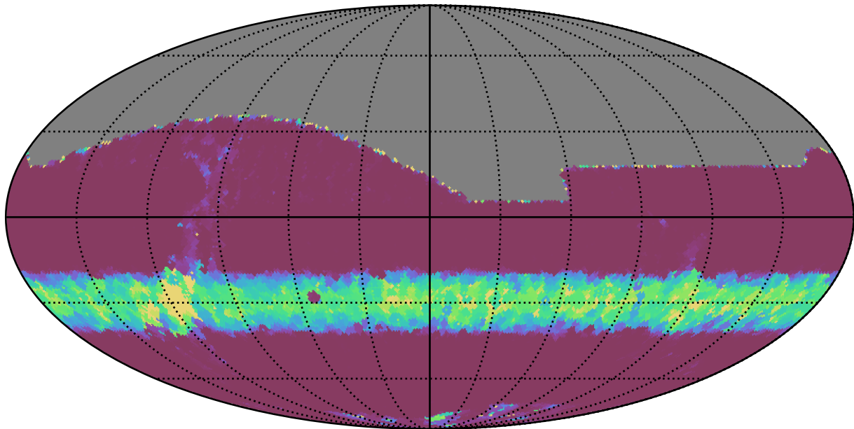
weather_cloudso8v3.4_10yrs All sky z band: Min normairmass
