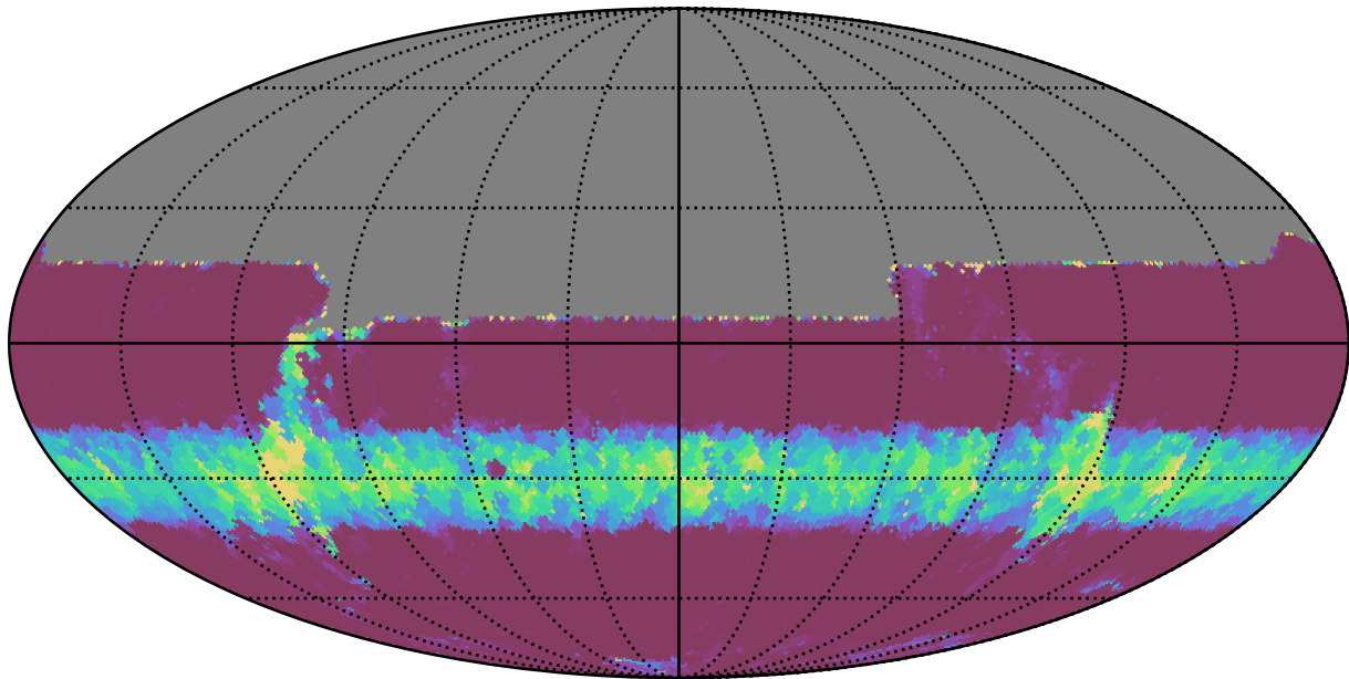
weather_cloudso8v3.4_10yrs All sky u band: Min normairmass
