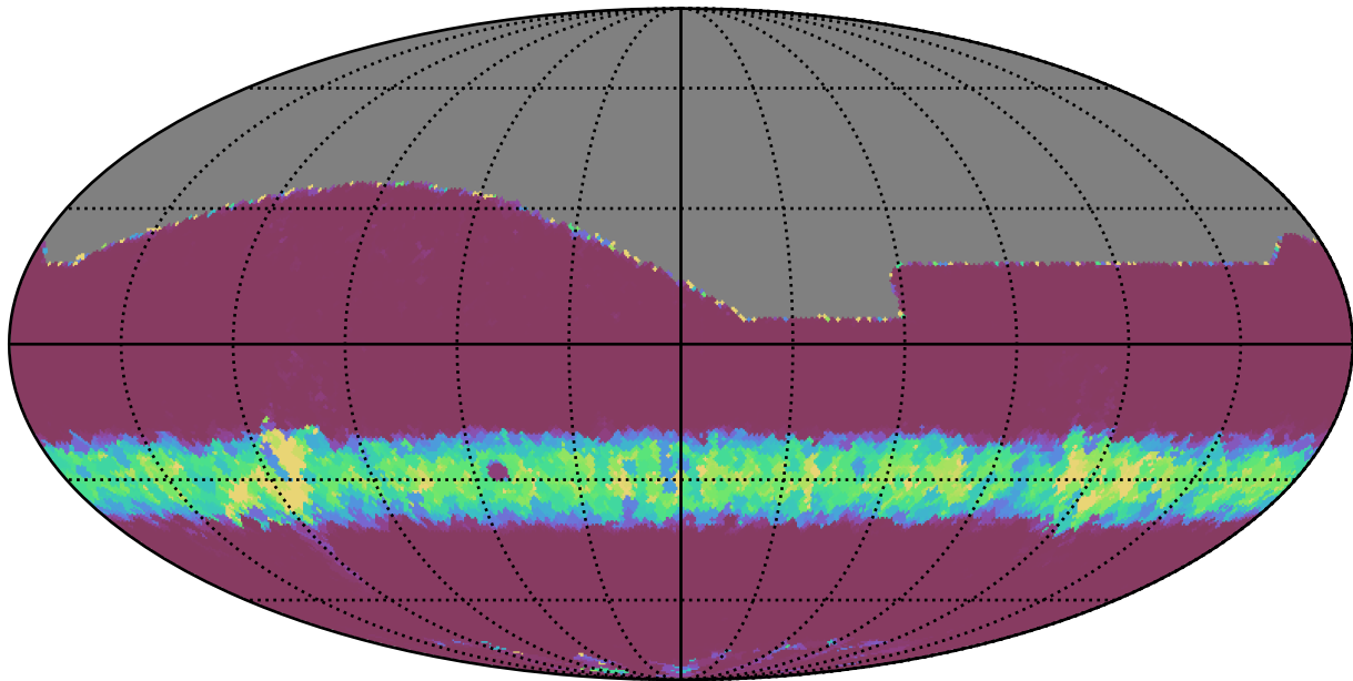
weather_cloudso8v3.4_10yrs All sky r band: Min normairmass
