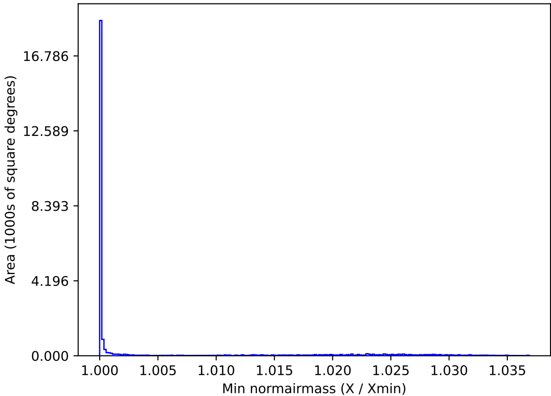
weather_cloudso8v3.4_10yrs All sky r band: Min normairmass
