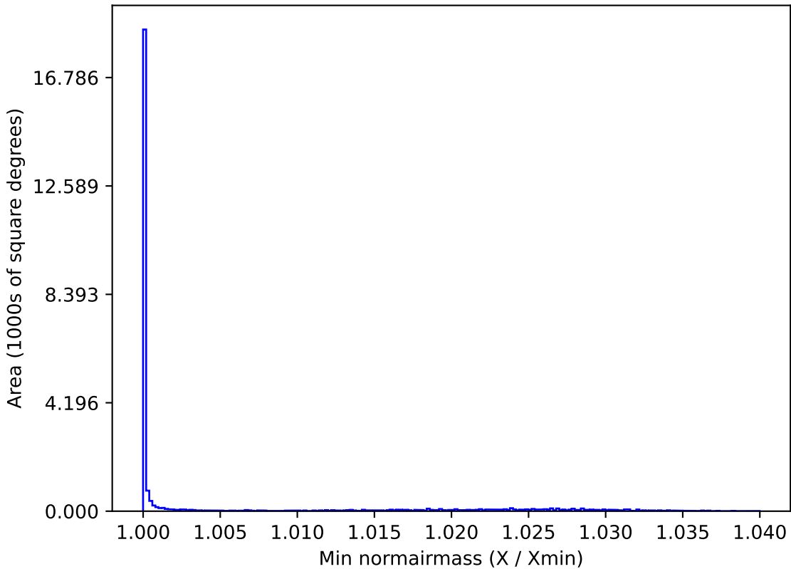
weather_cloudso8v3.4_10yrs All sky i band: Min normairmass
