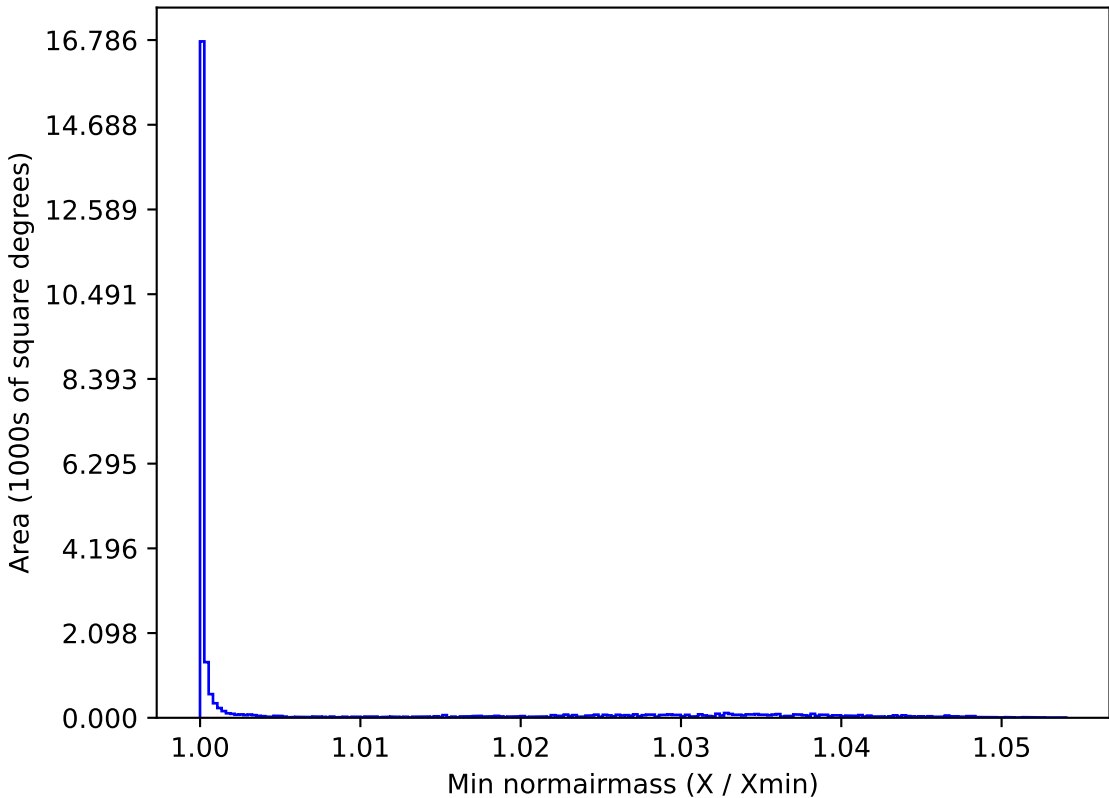
weather_cloudso8v3.4_10yrs All sky g band: Min normairmass
