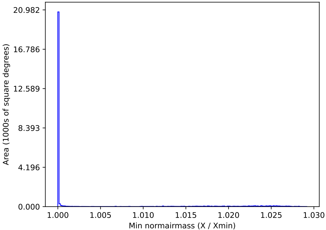
weather_cloudso8v3.4_10yrs All sky all bands: Min normairmass
