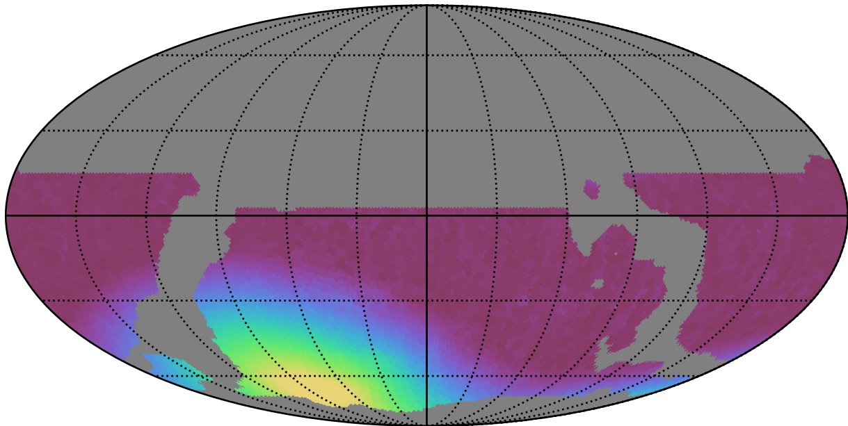
weather_cloudso8v3.4_10yrs WFD z band: Min moonDistance
