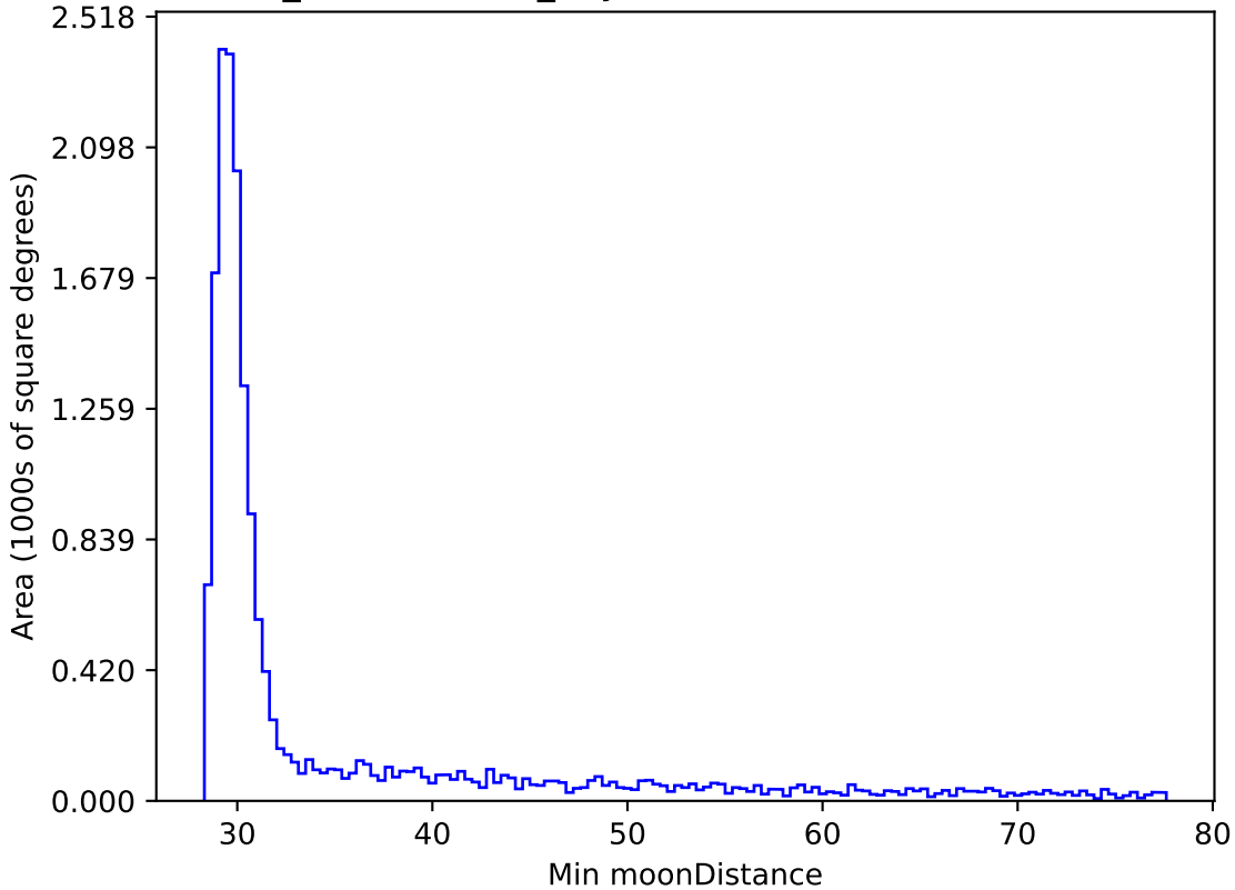
weather_cloudso8v3.4_10yrs WFD z band: Min moonDistance
