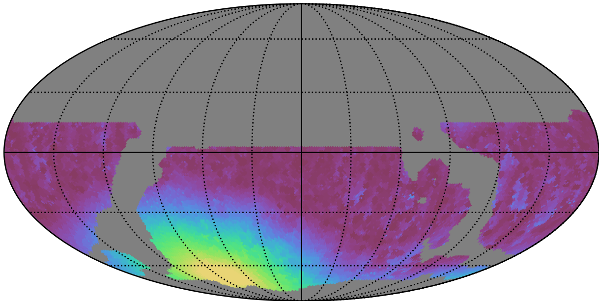
weather_cloudso8v3.4_10yrs WFD r band: Min moonDistance
