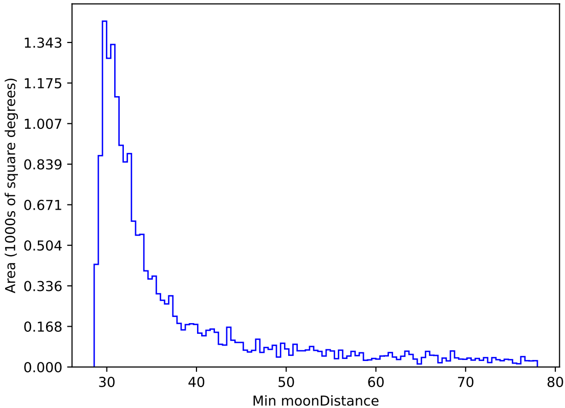
weather_cloudso8v3.4_10yrs WFD r band: Min moonDistance
