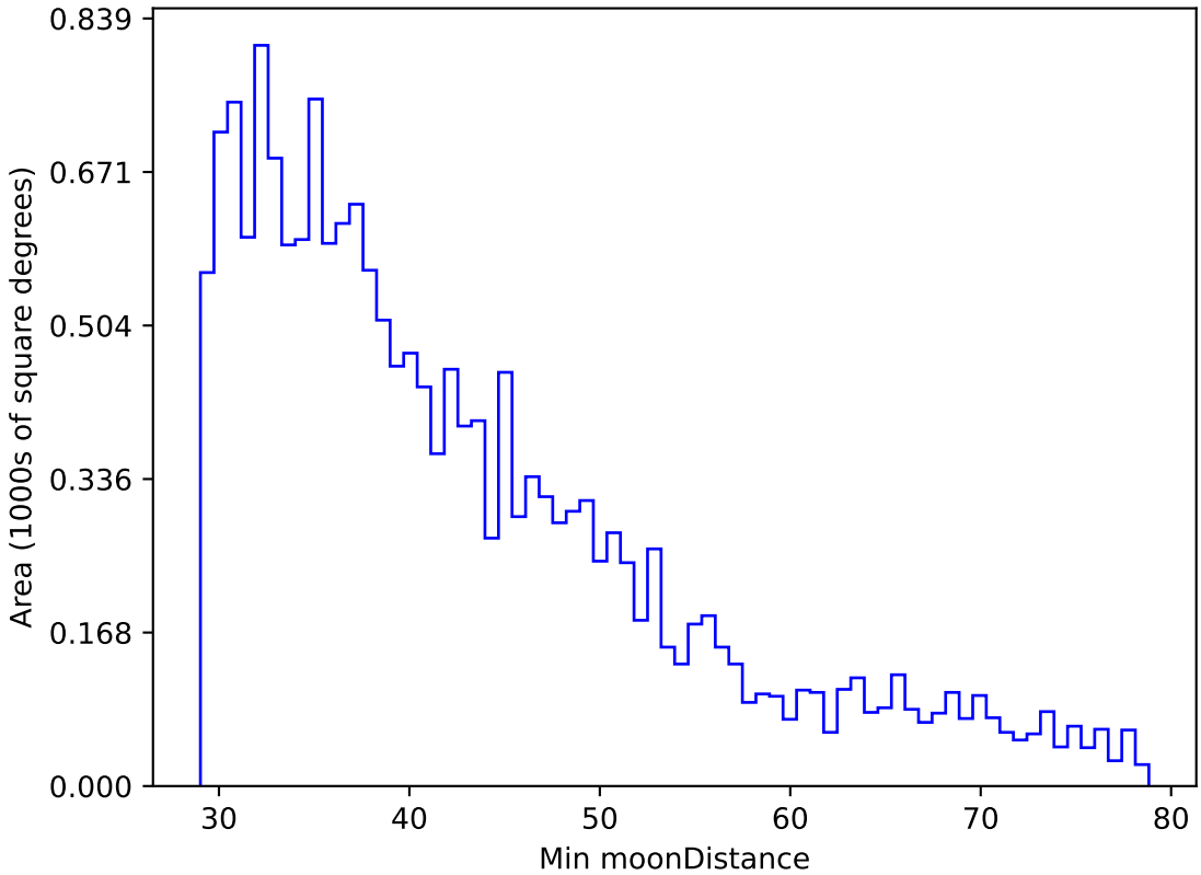
weather_cloudso8v3.4_10yrs WFD g band: Min moonDistance
