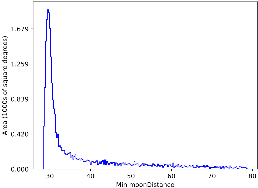
weather_cloudso8v3.4_10yrs All sky z band: Min moonDistance
