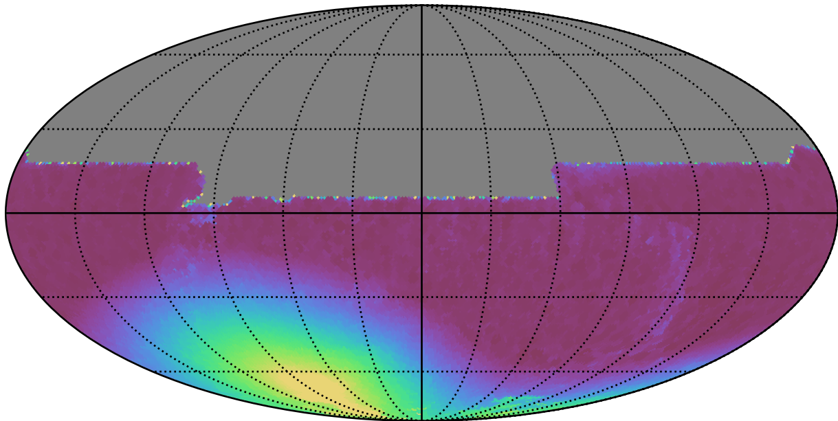
weather_cloudso8v3.4_10yrs All sky y band: Min moonDistance
