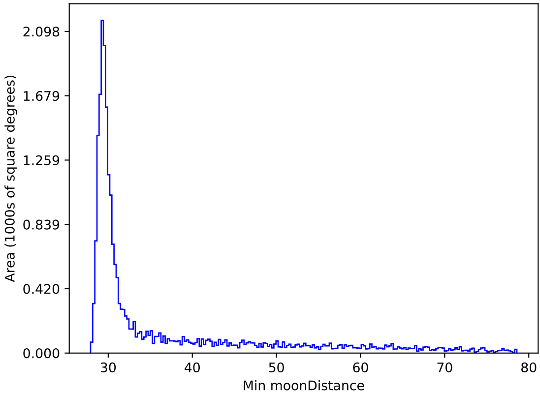
weather_cloudso8v3.4_10yrs All sky y band: Min moonDistance
