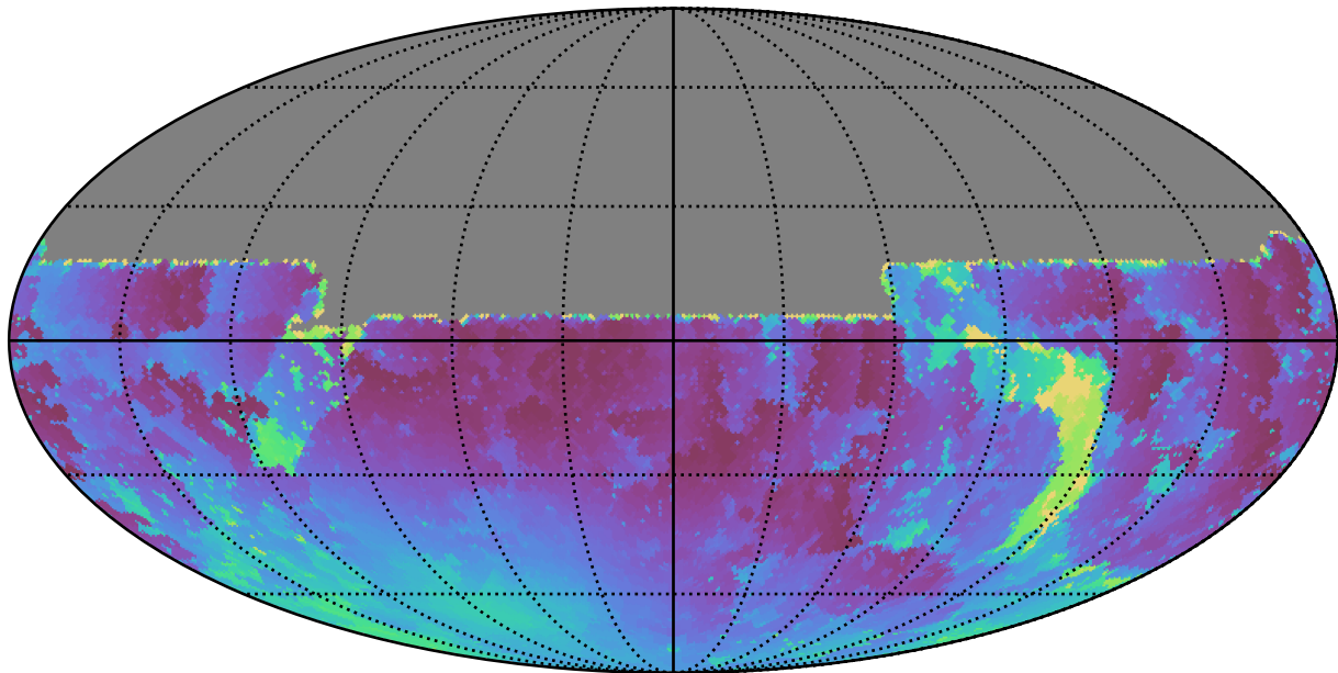
weather_cloudso8v3.4_10yrs All sky u band: Min moonDistance
