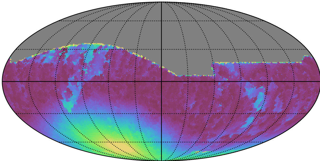
weather_cloudso8v3.4_10yrs All sky r band: Min moonDistance
