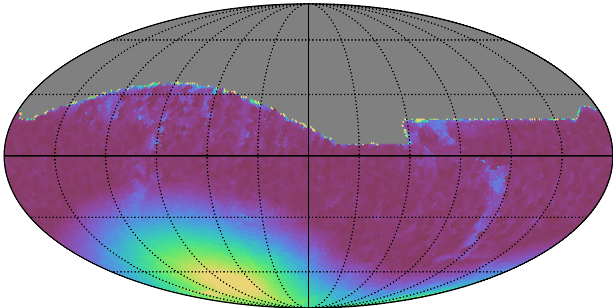
weather_cloudso8v3.4_10yrs All sky i band: Min moonDistance
