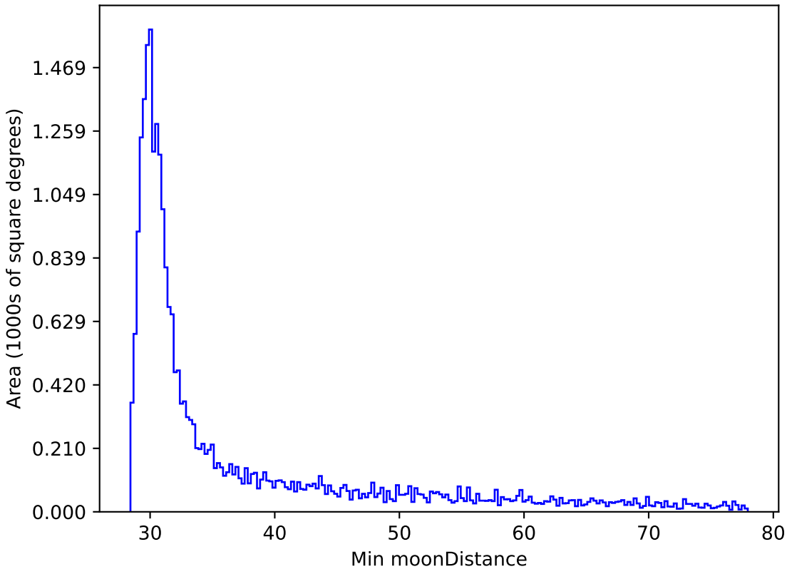
weather_cloudso8v3.4_10yrs All sky i band: Min moonDistance
