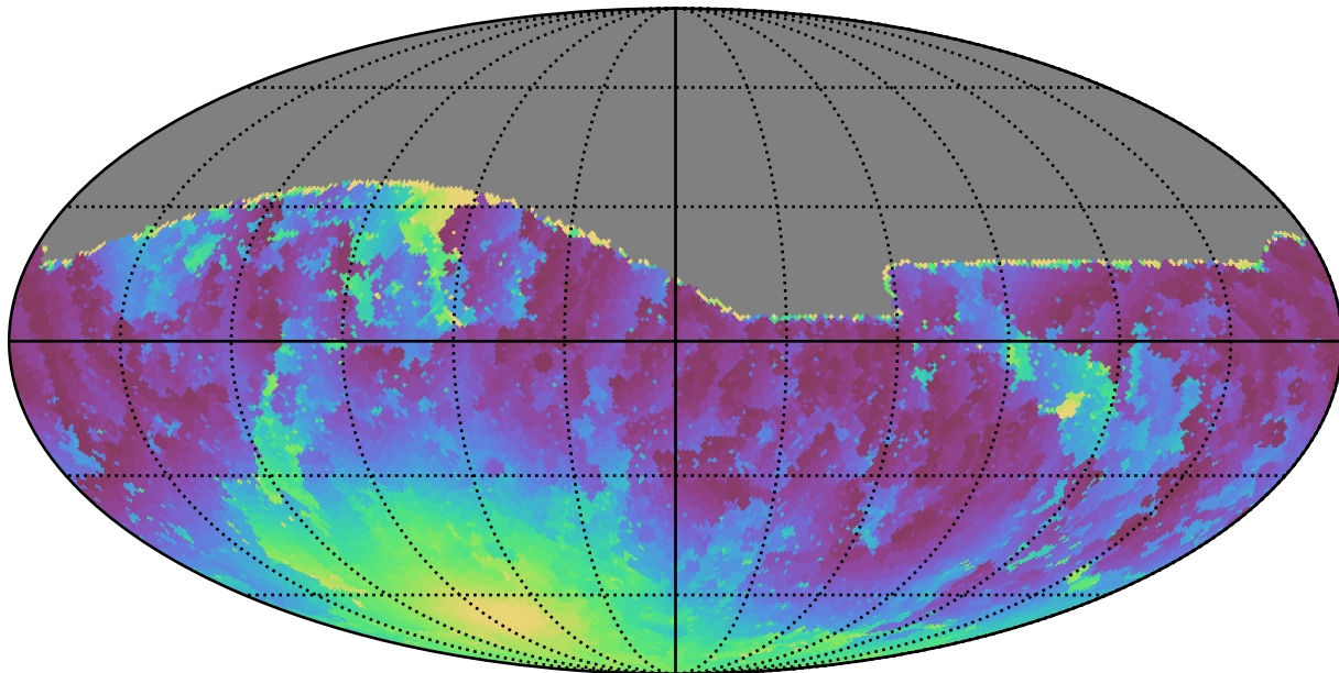
weather_cloudso8v3.4_10yrs All sky g band: Min moonDistance
