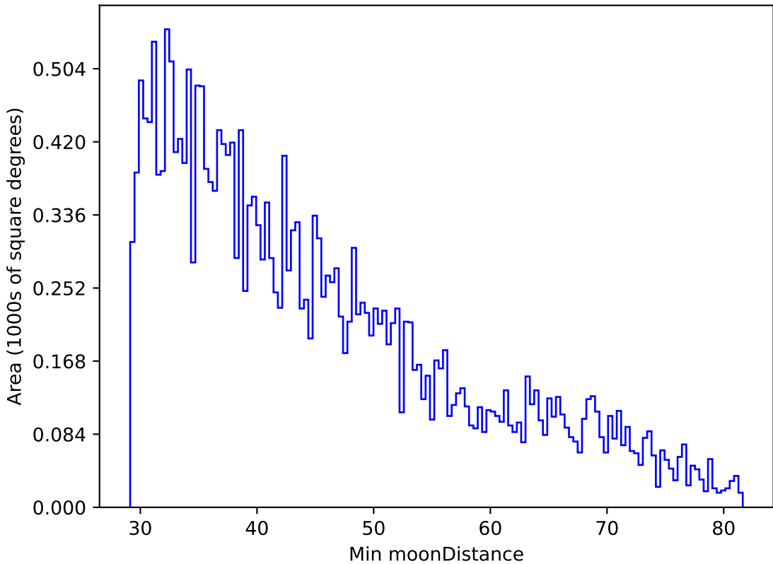
weather_cloudso8v3.4_10yrs All sky g band: Min moonDistance
