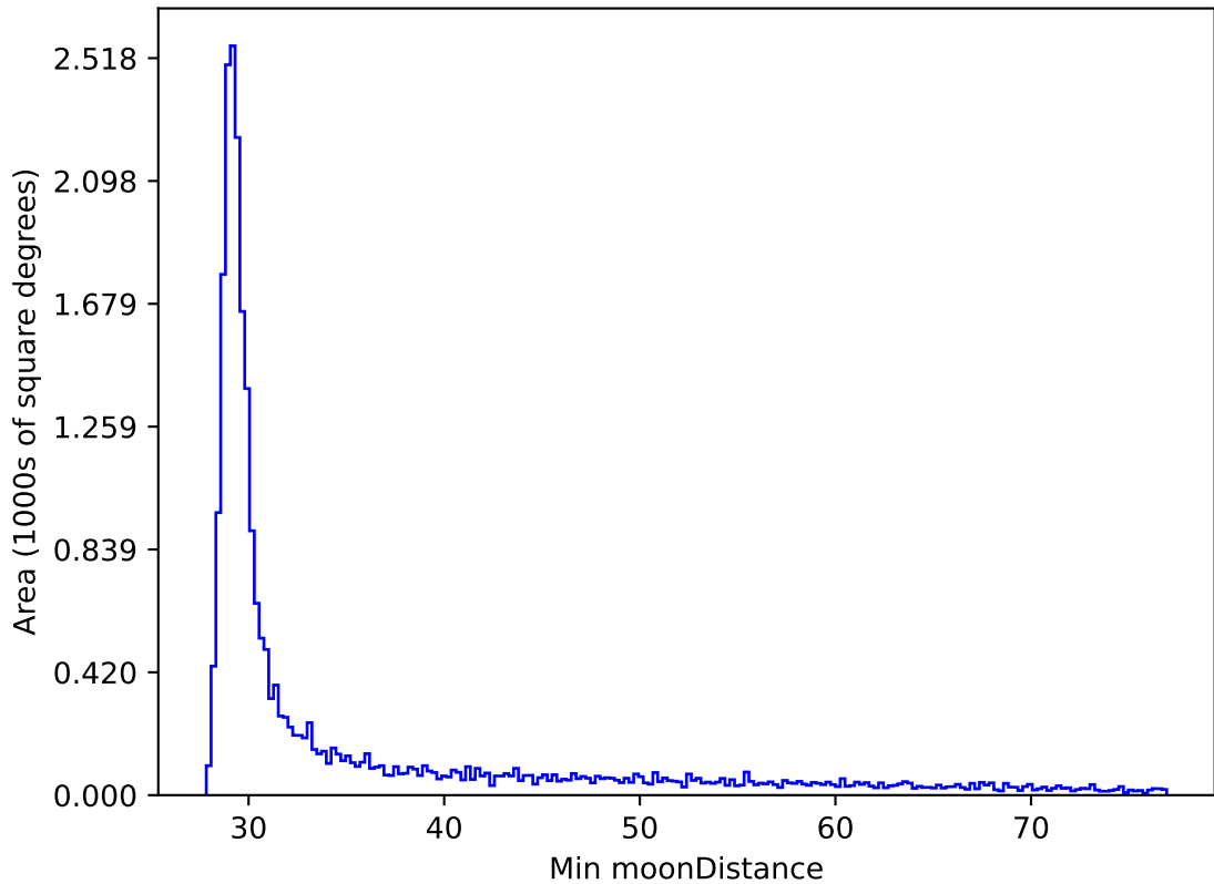
weather_cloudso8v3.4_10yrs All sky all bands: Min moonDistance
