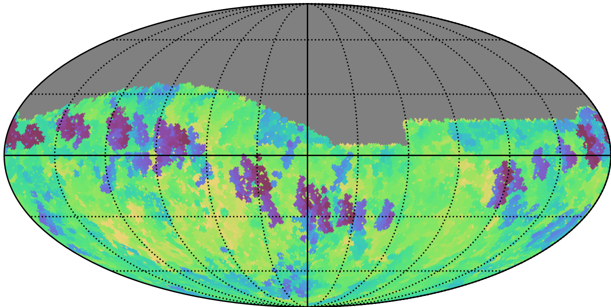
weather_cloudso8v3.4_10yrs Yr 1 z band: Min fiveSigmaDepth
