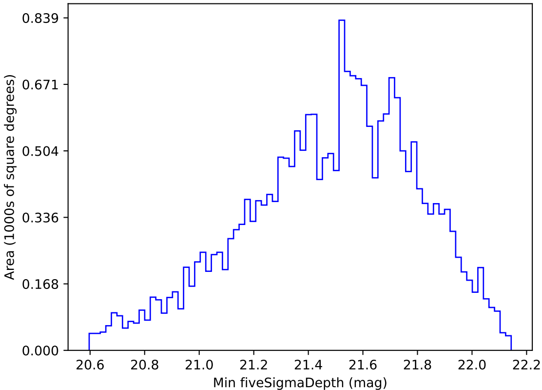
weather_cloudso8v3.4_10yrs Yr 1 y band: Min fiveSigmaDepth
