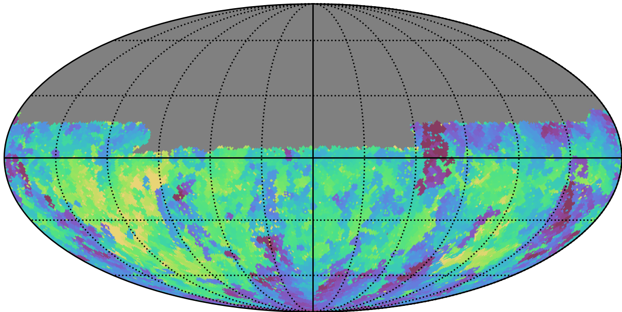
weather_cloudso8v3.4_10yrs Yr 1 u band: Min fiveSigmaDepth
