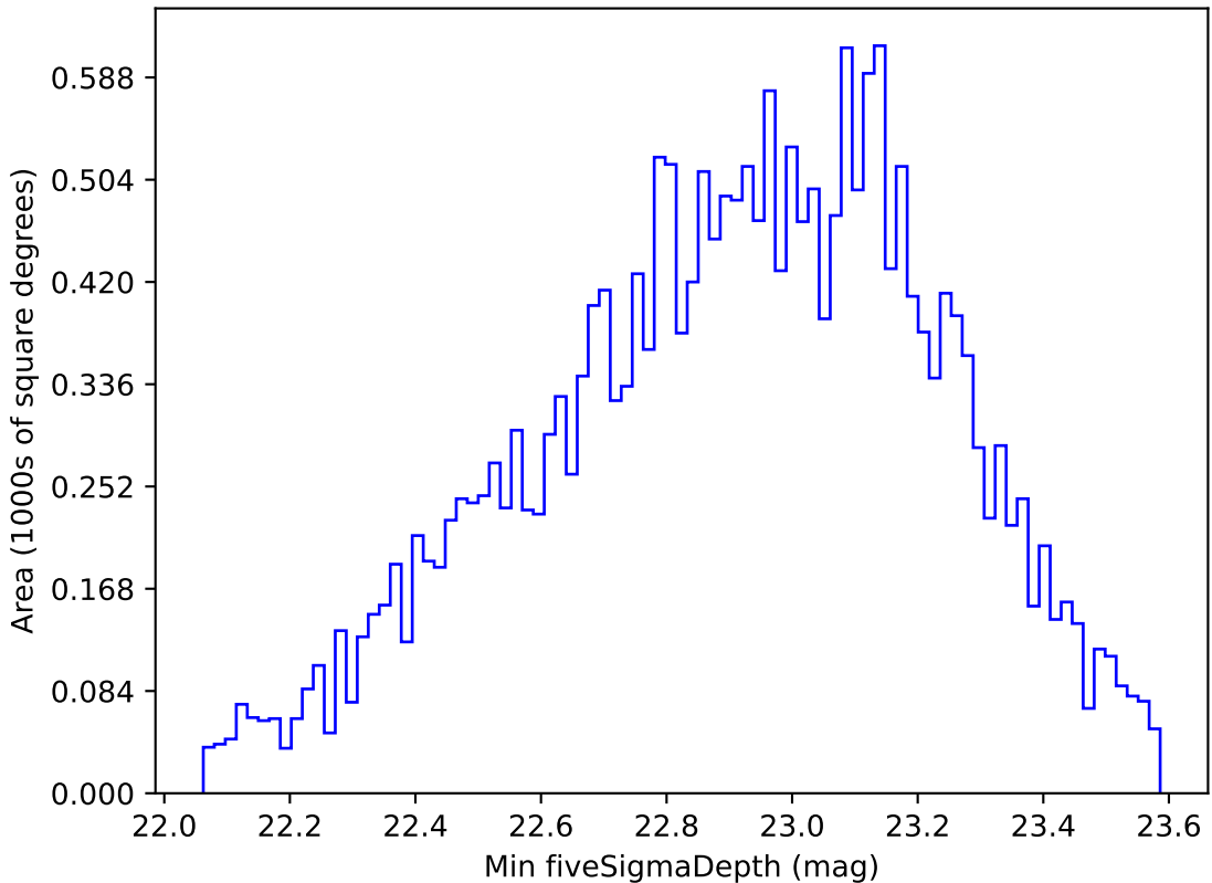
weather_cloudso8v3.4_10yrs Yr 1 u band: Min fiveSigmaDepth
