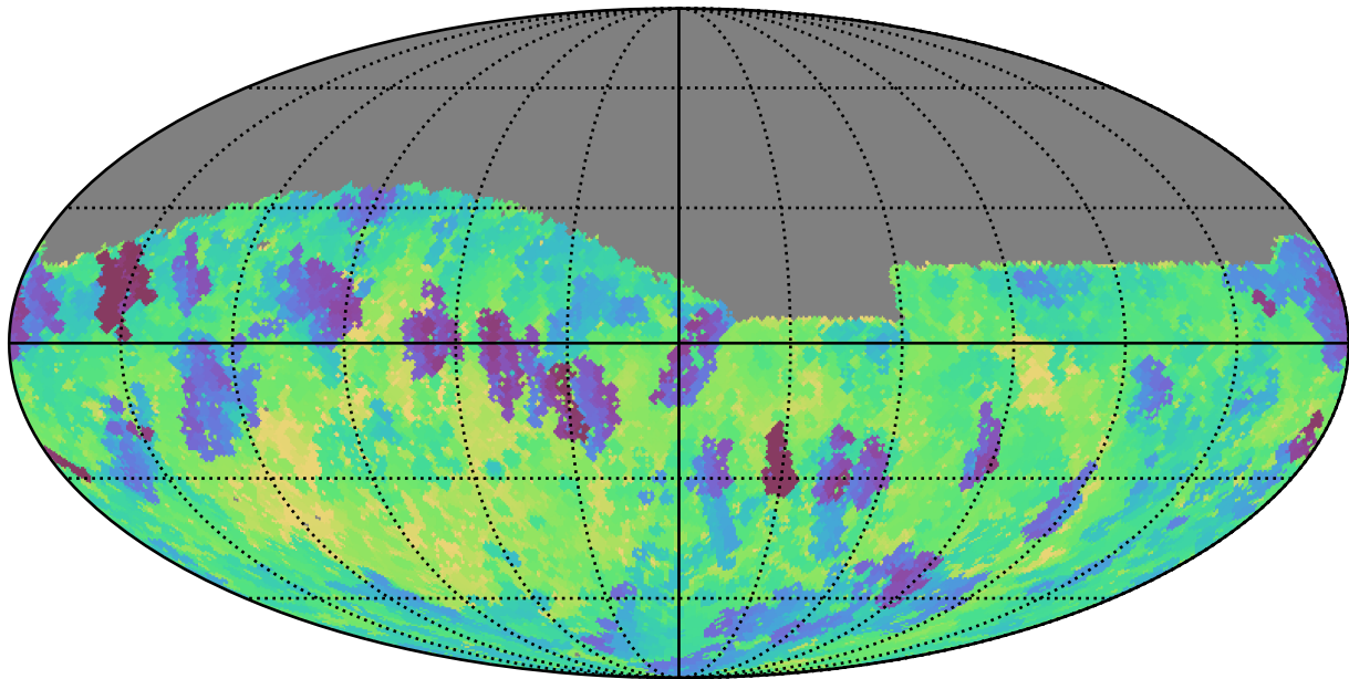
weather_cloudso8v3.4_10yrs Yr 1 i band: Min fiveSigmaDepth
