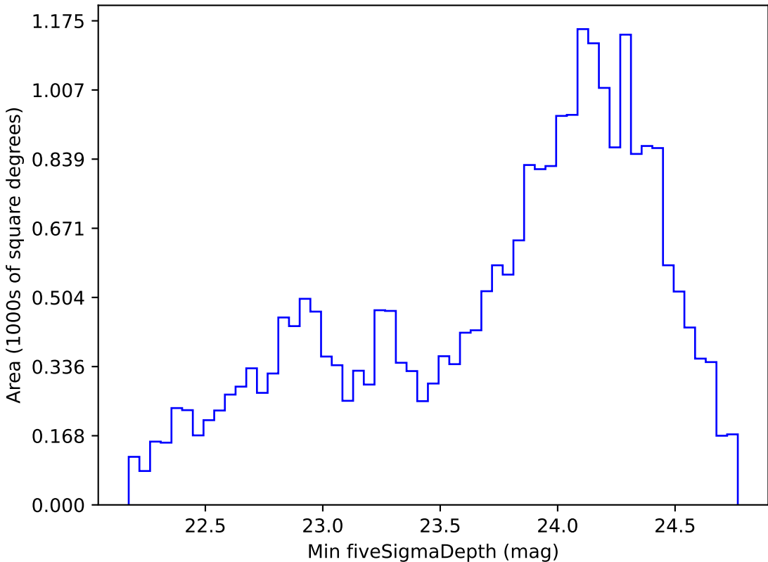
weather_cloudso8v3.4_10yrs Yr 1 g band: Min fiveSigmaDepth
