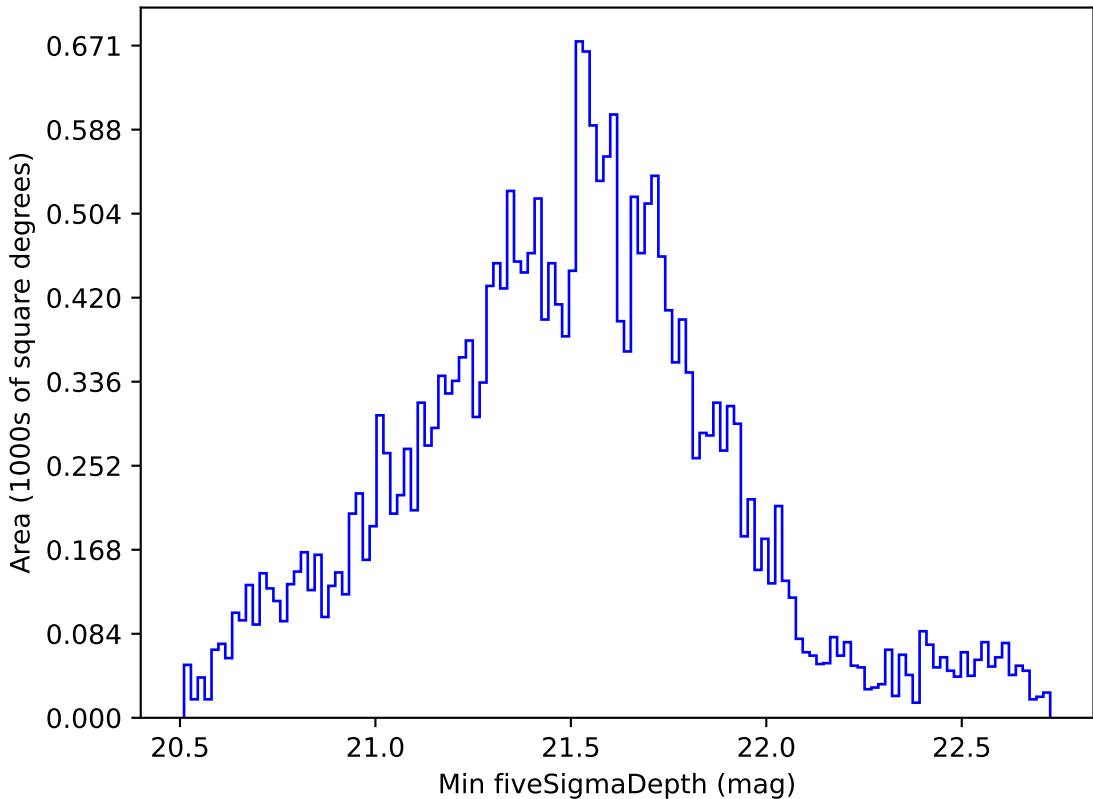
weather_cloudso8v3.4_10yrs Yr 1 all bands: Min fiveSigmaDepth
