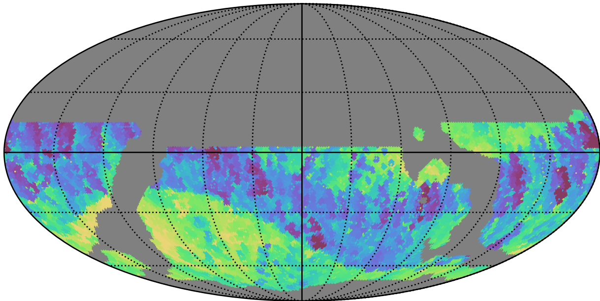
weather_cloudso8v3.4_10yrs WFD z band: Min fiveSigmaDepth
