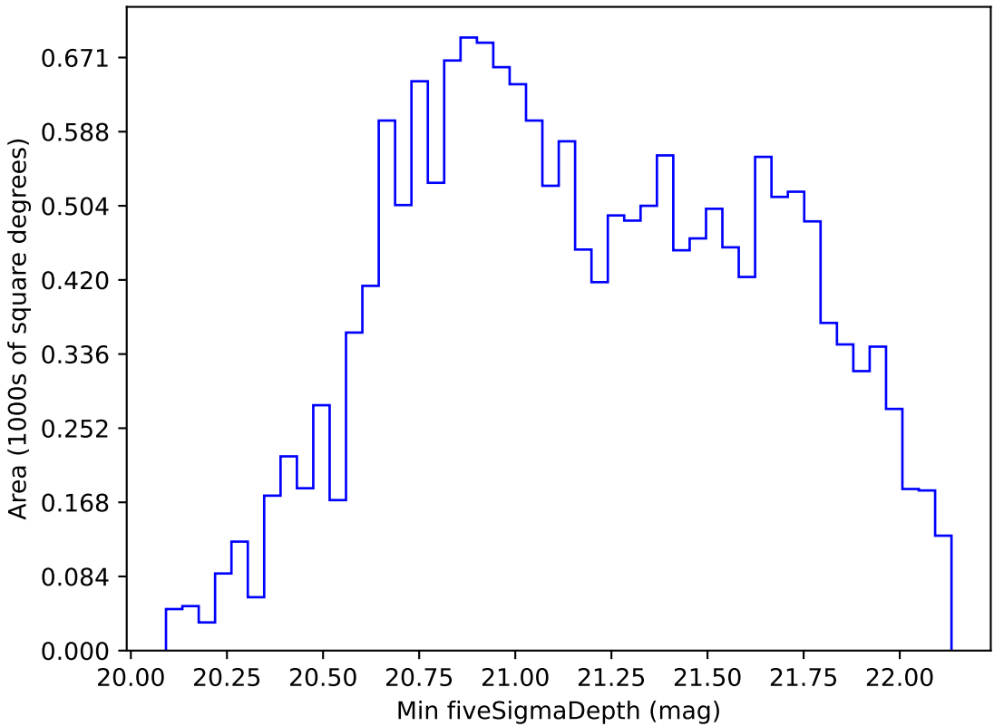
weather_cloudso8v3.4_10yrs WFD z band: Min fiveSigmaDepth
