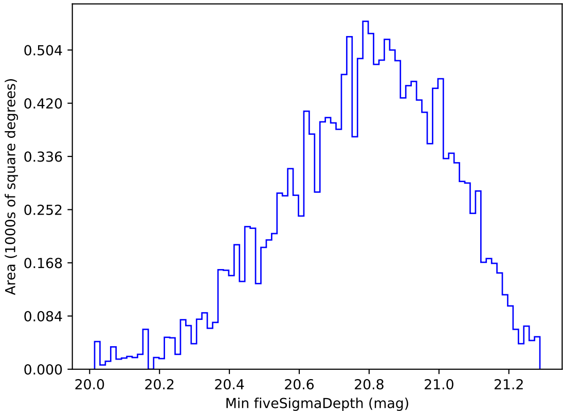
weather_cloudso8v3.4_10yrs WFD y band: Min fiveSigmaDepth
