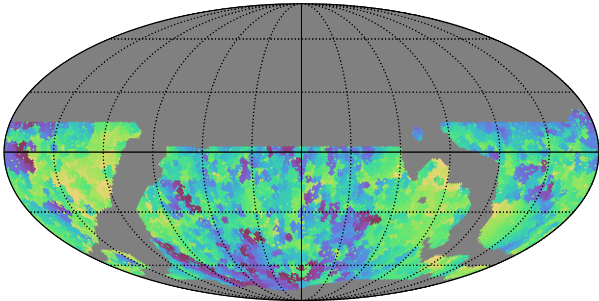
weather_cloudso8v3.4_10yrs WFD u band: Min fiveSigmaDepth
