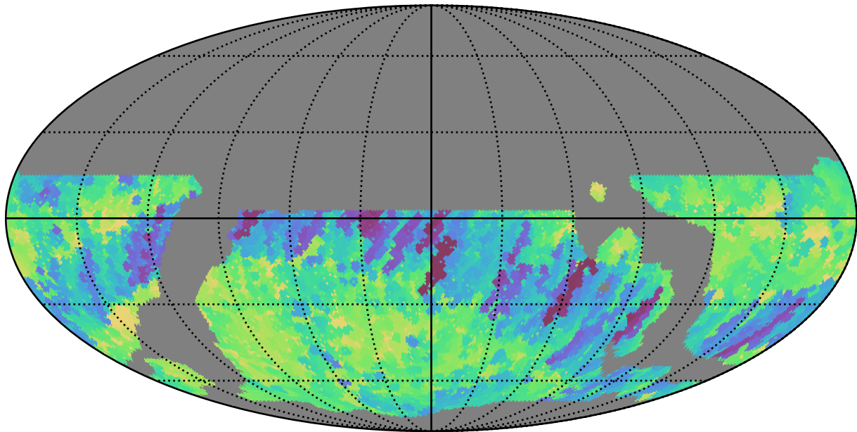
weather_cloudso8v3.4_10yrs WFD r band: Min fiveSigmaDepth
