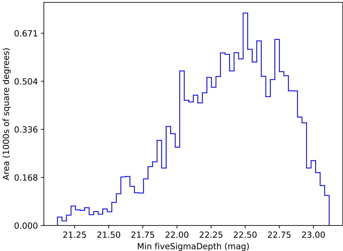
weather_cloudso8v3.4_10yrs WFD r band: Min fiveSigmaDepth
