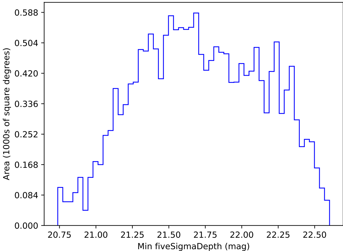
weather_cloudso8v3.4_10yrs WFD i band: Min fiveSigmaDepth
