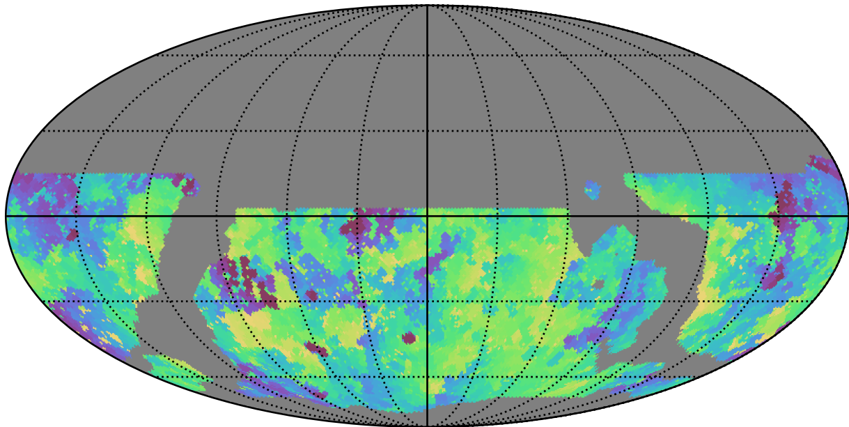
weather_cloudso8v3.4_10yrs WFD g band: Min fiveSigmaDepth
