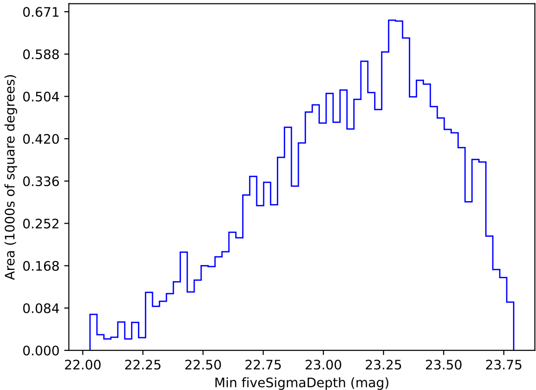
weather_cloudso8v3.4_10yrs WFD g band: Min fiveSigmaDepth
