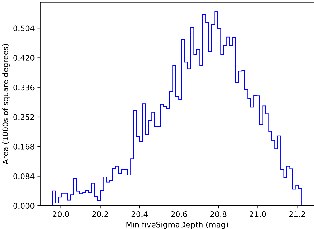
weather_cloudso8v3.4_10yrs WFD all bands: Min fiveSigmaDepth
