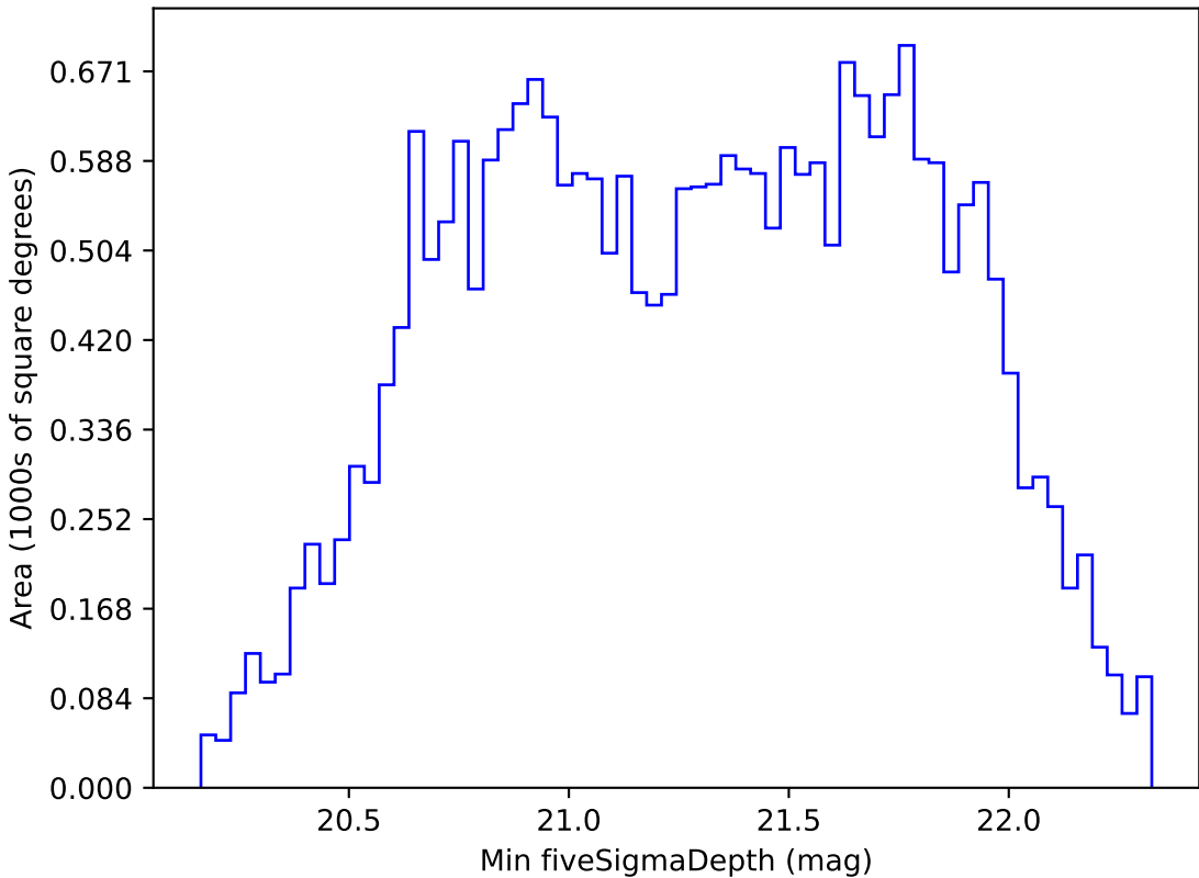
weather_cloudso8v3.4_10yrs All sky z band: Min fiveSigmaDepth
