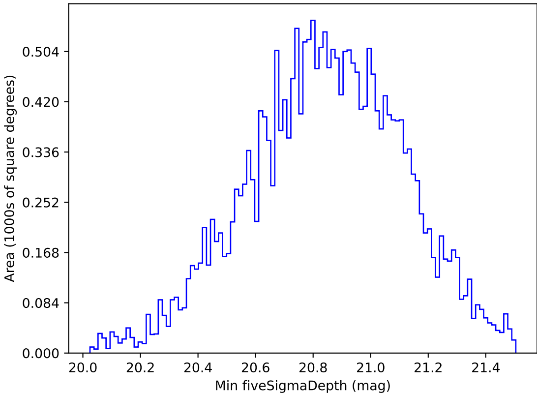
weather_cloudso8v3.4_10yrs All sky y band: Min fiveSigmaDepth
