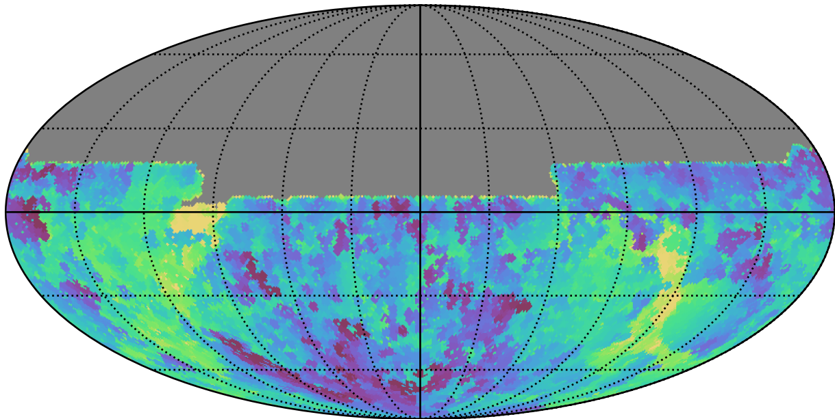
weather_cloudso8v3.4_10yrs All sky u band: Min fiveSigmaDepth
