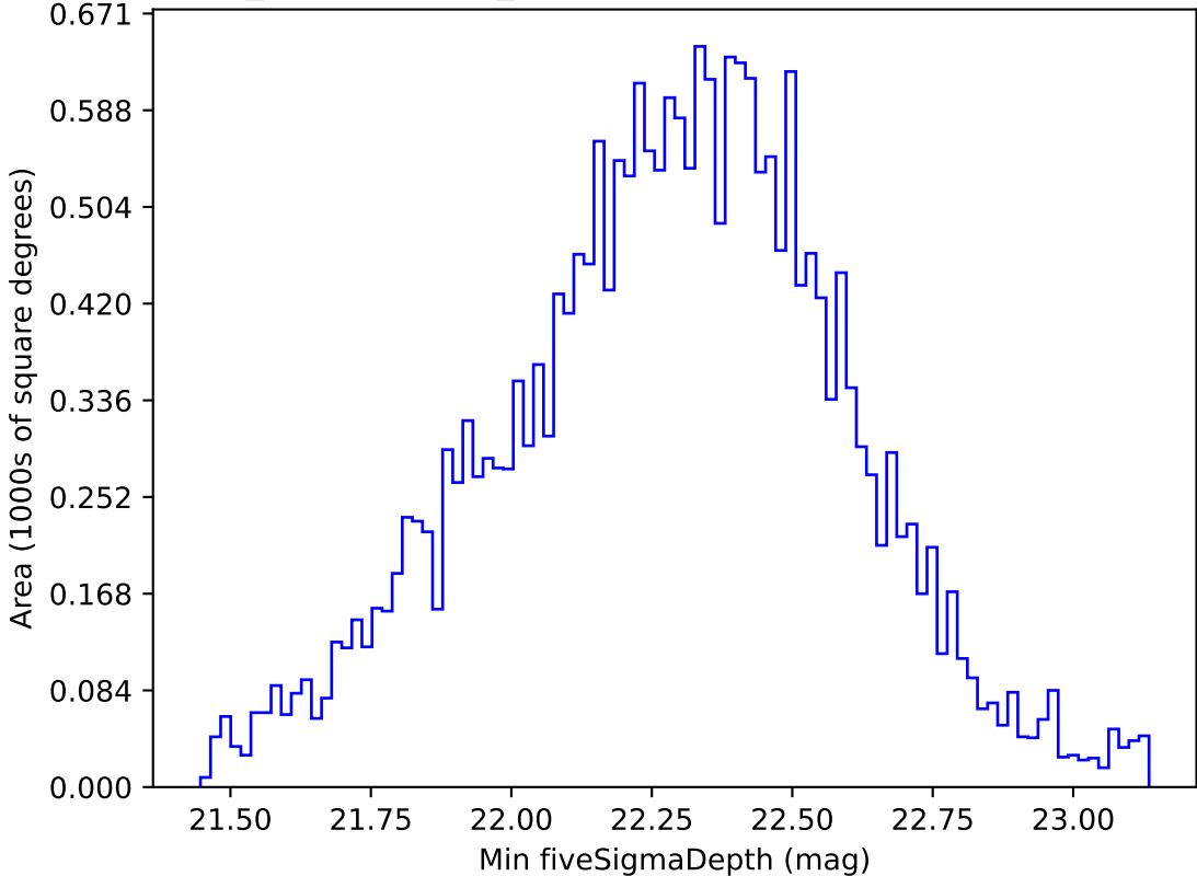
weather_cloudso8v3.4_10yrs All sky u band: Min fiveSigmaDepth
