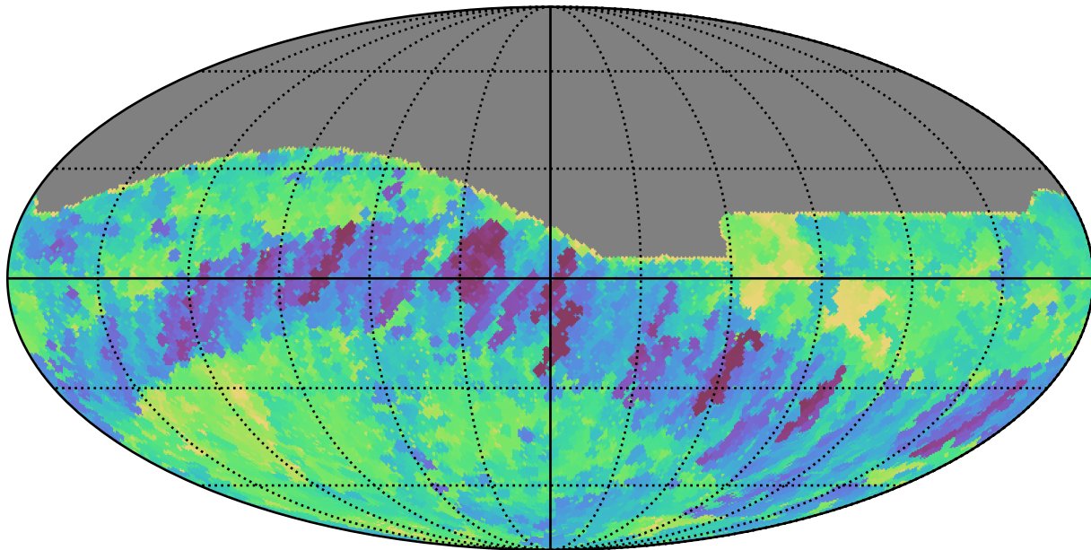
weather_cloudso8v3.4_10yrs All sky r band: Min fiveSigmaDepth
