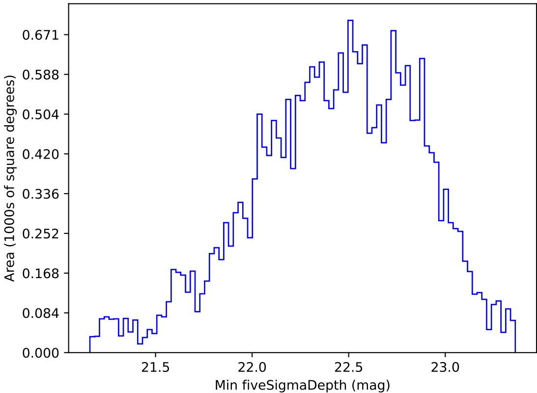
weather_cloudso8v3.4_10yrs All sky r band: Min fiveSigmaDepth
